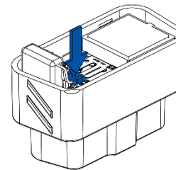
3 Figure 5 Battery connection
