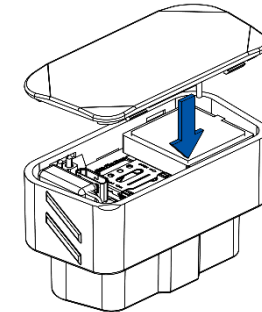
4 Figure 6 Attach device cover back
